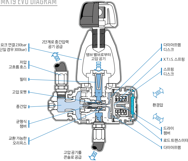
MK19 EVO DIAGRAM
