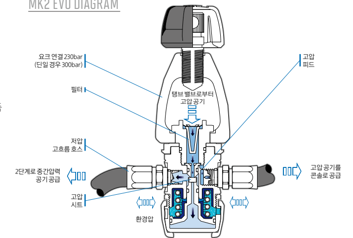
MK2 EVO DIAGRAM
