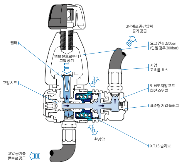
MK25 EVO DIAGRAM
